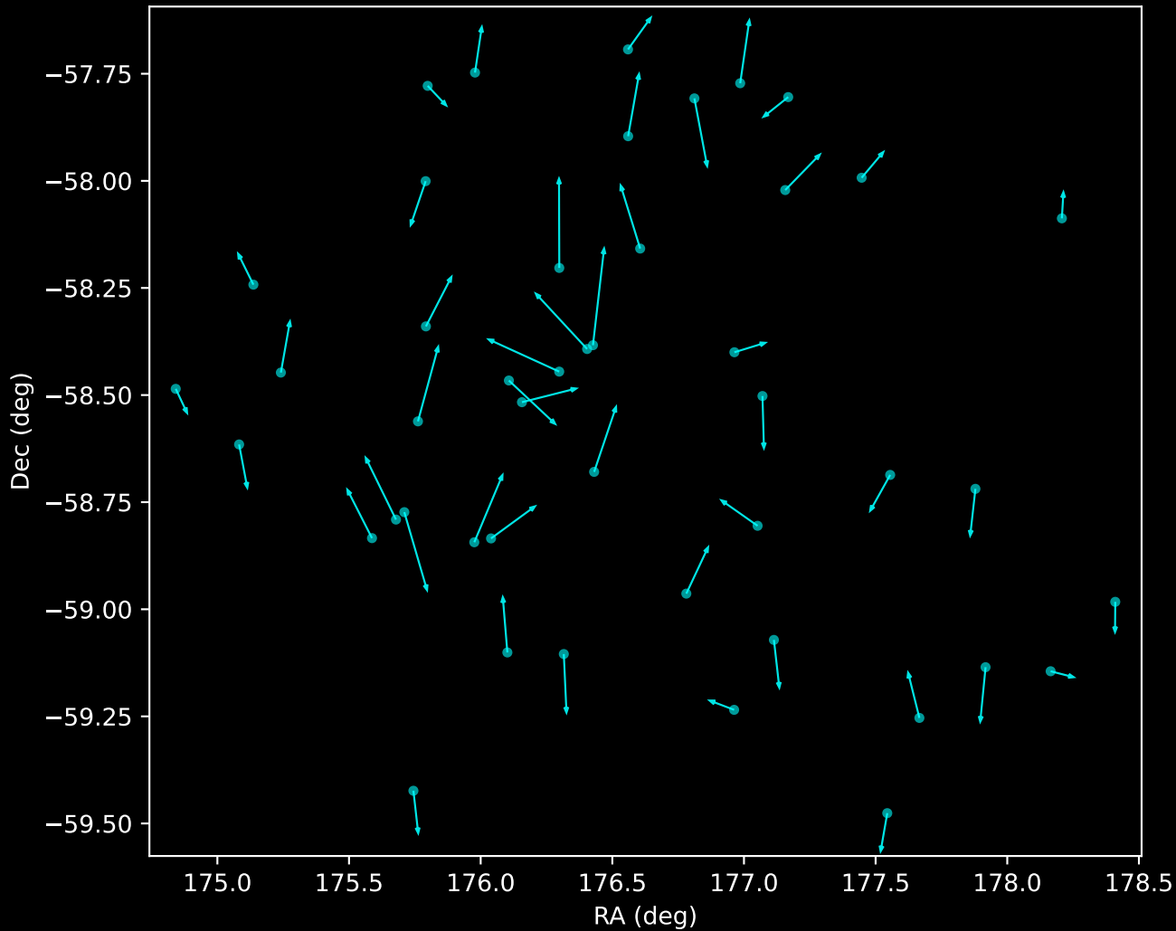
GALAH DR4 Noise Stream Proper Motion Vectors (n=46)
