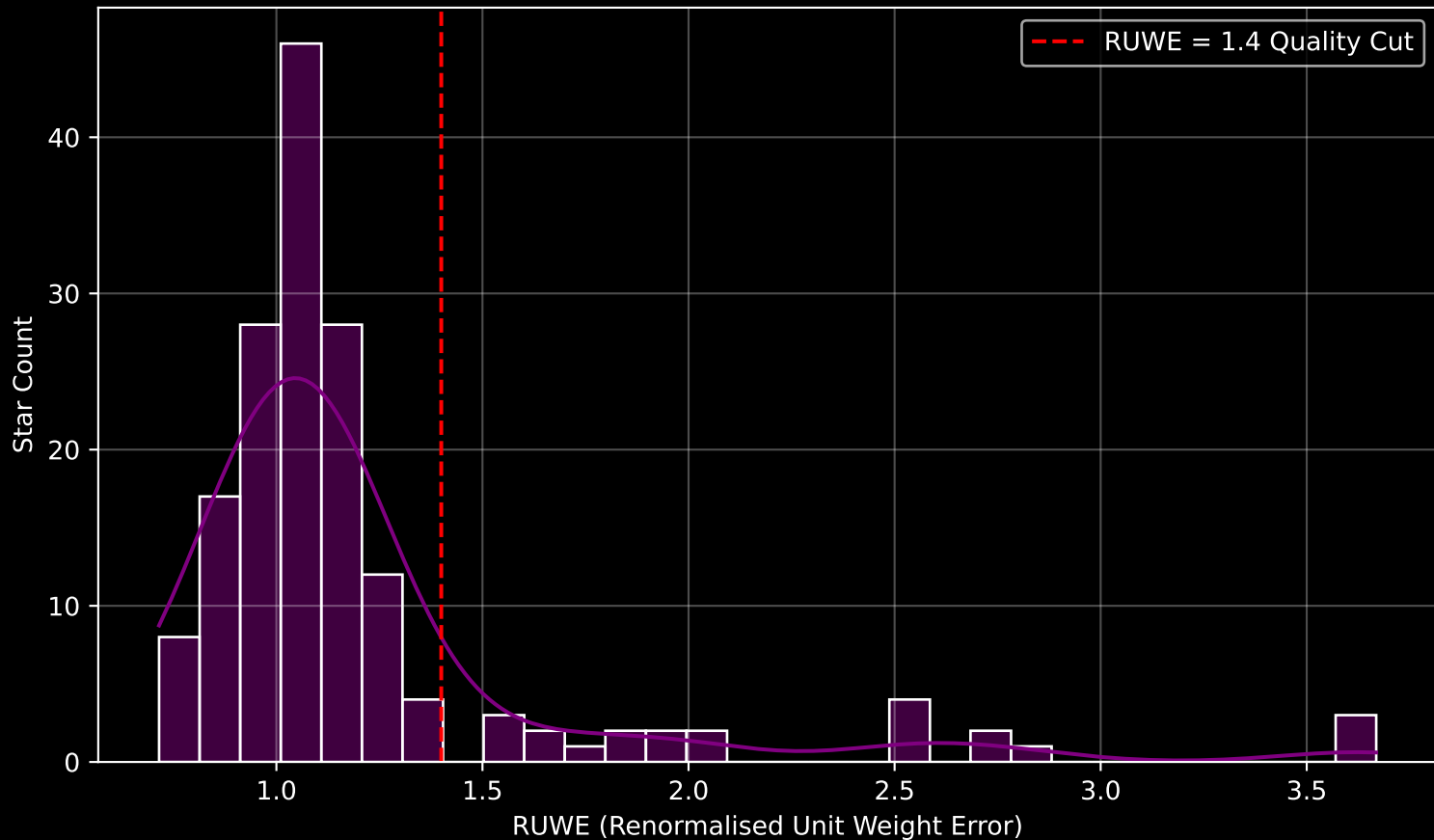
GALAH DR4 Field [7183] RUWE Distribution (n= 165)
