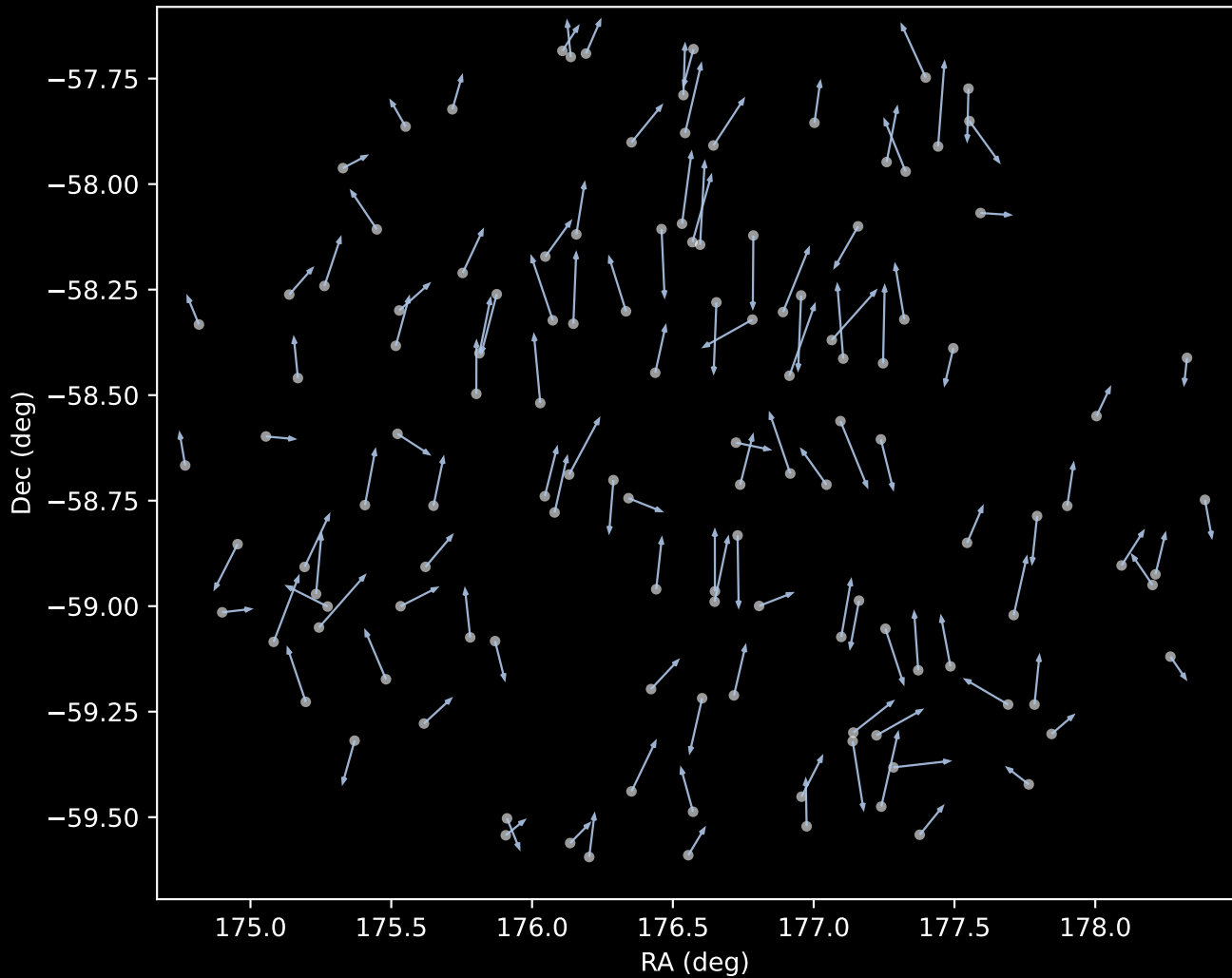
GALAH DR4 Cluster 1 Proper Motion Vectors (n=127)
