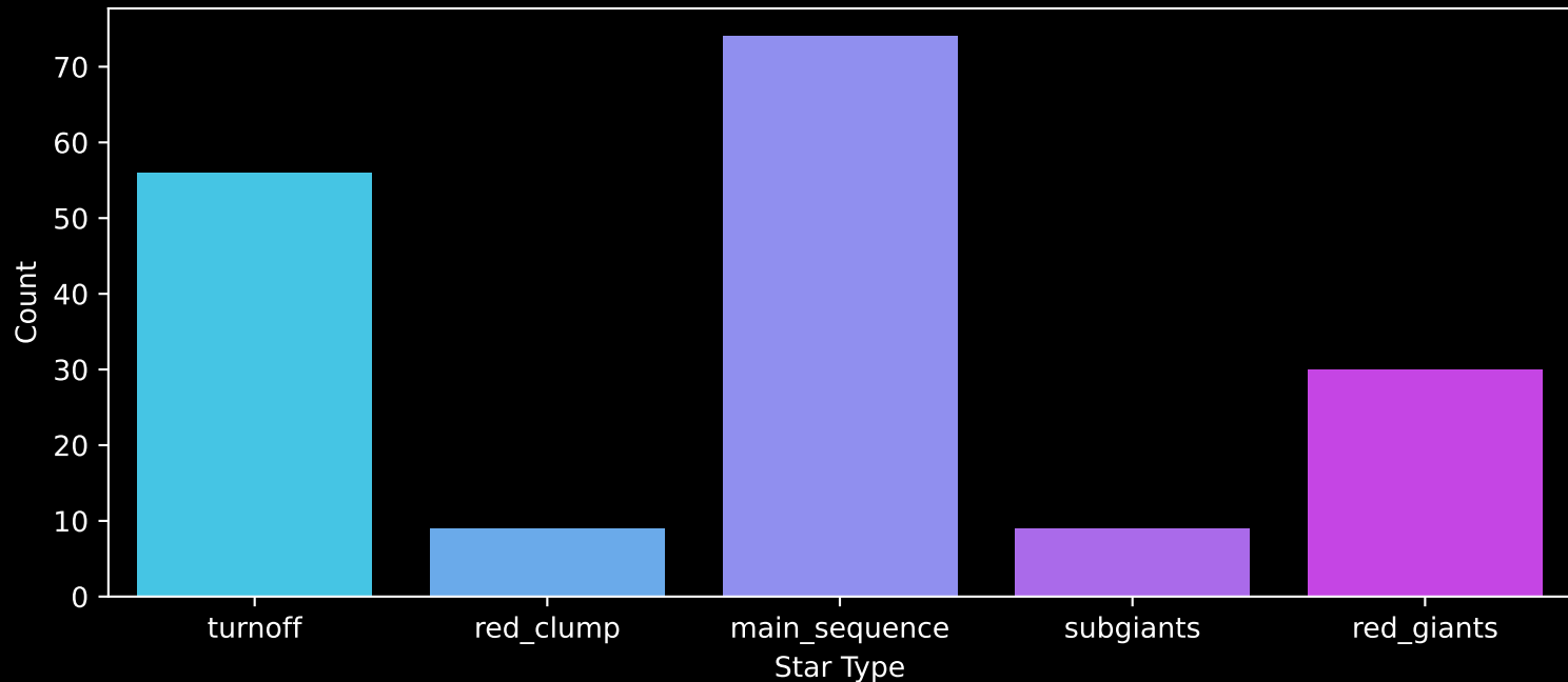
GALAH DR4 Field: [7183] Count plot of Star Type
