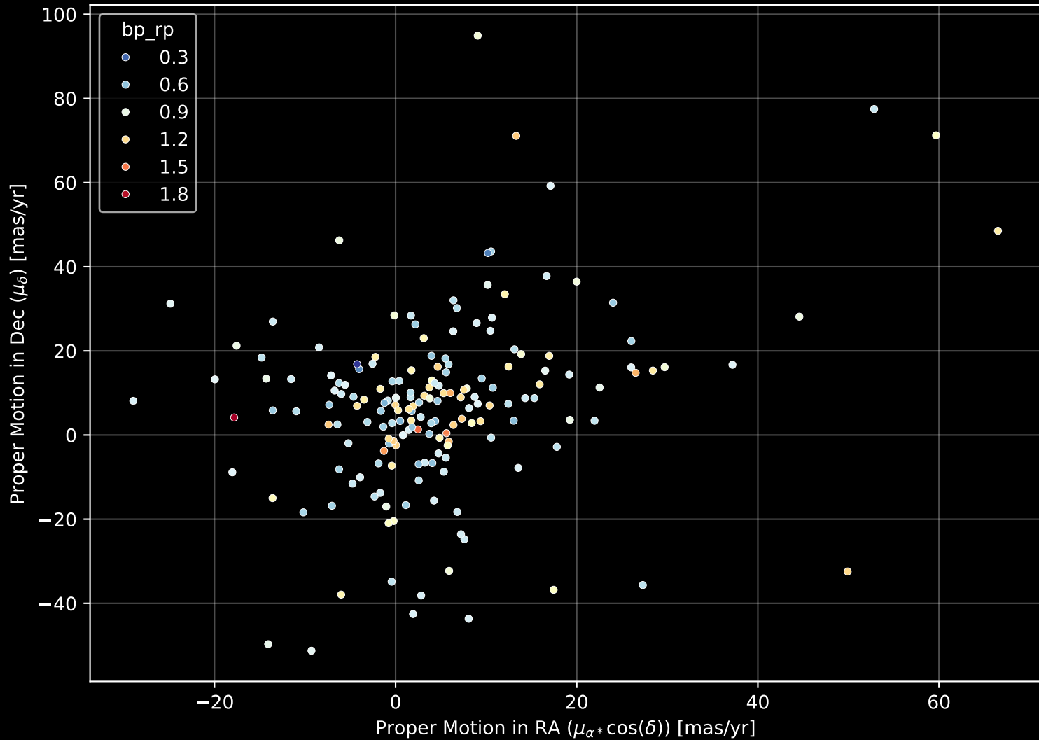
GALAH DR4 Field: [7183] Proper Motion Diagram (n= 178)
